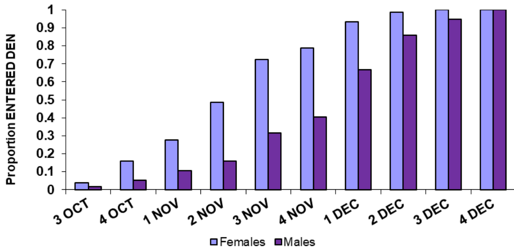
Figure 17. Cumulative proportion of den entries for female and male, radio-collared grizzly bears in the Cabinet-Yaak grizzly bear recovery zone, by month and week, 1983–2021.
