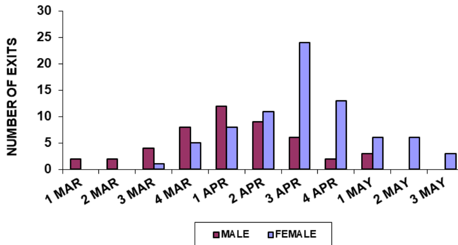
Figure 18. Month and week of den exit for male and female radio-collared grizzly bears in the Cabinet-Yaak grizzly bear recovery zone, 1983–2021.
