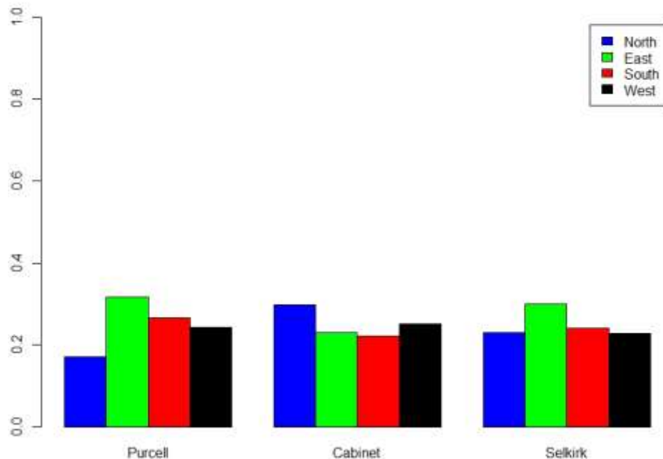
Figure 21. Yearly proportional use of aspect for grizzly bear VHF and GPS locations in the Yaak River from 1986–2021, the Cabinet Mountains from 1986–2021, and the Selkirk Mountains from 1986–2021.
