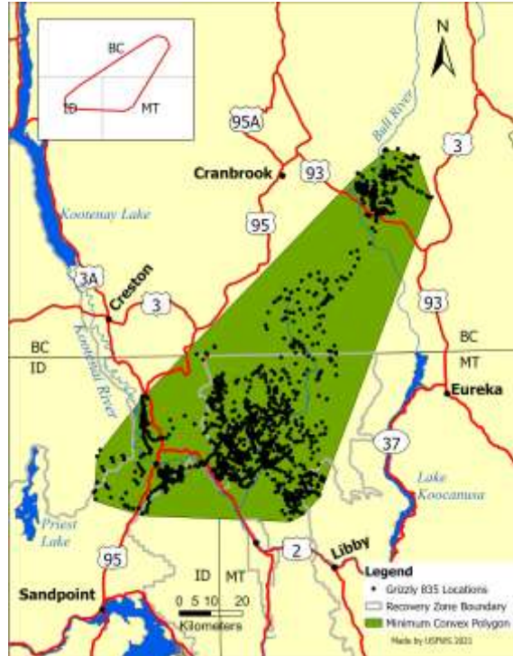
Figure A76. Radio locations and minimum convex (shaded) life range of male grizzly bear 835 in the Yaak River, 2014–2016, 2019–2021.
