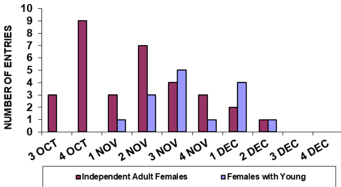
Figure 16. Month and week of den entry for adult female, radio-collared grizzly bears in the Cabinet-Yaak grizzly bear recovery zone, 1983–2021.
