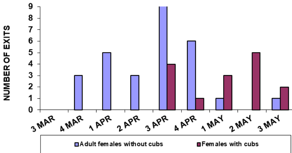
Figure 19. Month and week of den exit for adult female, radio-collared grizzly bears (with and without cubs) in the Cabinet-Yaak grizzly bear recovery zone, 1983–2021.
