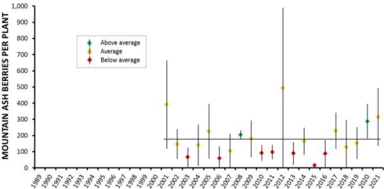
Figure 29. Mean berries per plant ( \pm 95% confidence interval) for mountain ash transects in the Cabinet-Yaak, 2001–2021. Horizontal line indicates study-wide mean production, 2001–2021.
