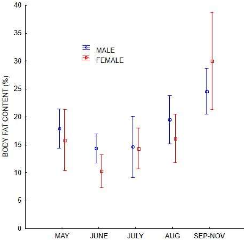
Figure 31. Mean percent body fat content (kg fat / kg body mass) of captured female and male grizzly bears in the Cabinet-Yaak and Selkirk mountains 2010–2019, by month. Error bars represent 95% confidence intervals.
